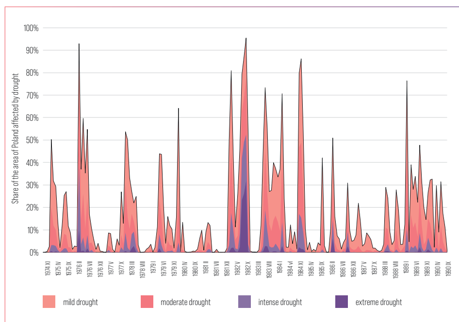
FIGURE 15 CHANGES IN THE INTENSITY AND SPATIAL EXTENT OF METEOROLOGICAL DROUGHT IN THE MULTIANNUL PERIOD OF 1975-1990 [SOURCE: SZALIŃSKA, TOKARCZYK, 2022]
