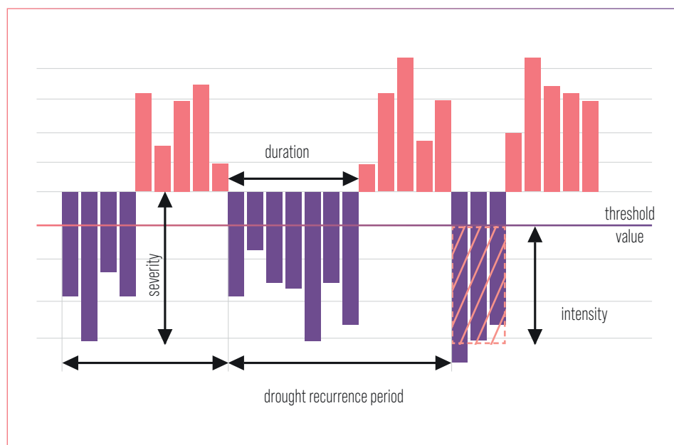
FIGURE 20 ELEMENTS OF DROUGHT HAZARD ASSESSMENT IN A GIVEN AREA: DURATION, INTENSITY, SEVERITY OF DROUGHT, RECURRENCE PERIOD [SOURCE: SZALIŃSKA, TOKARCZYK, 2022]
